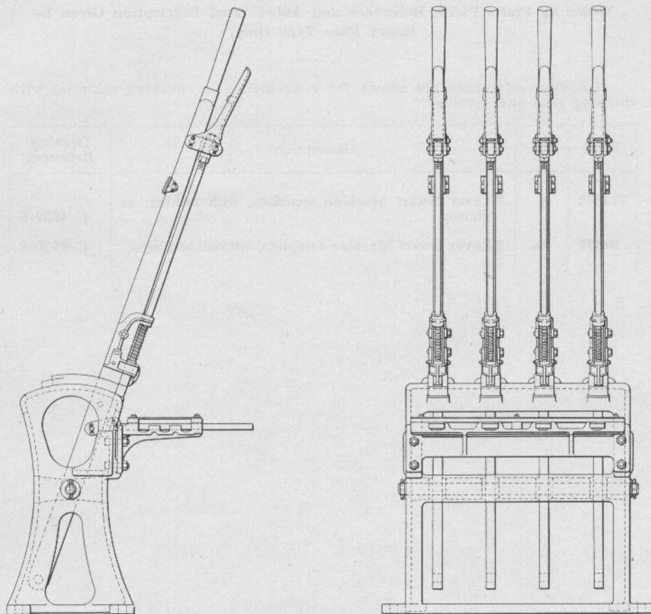
THE DWARF INTERLOCKING MACHINE ARRANGED FOR CONNECTIONS ABOVE FLOOR
